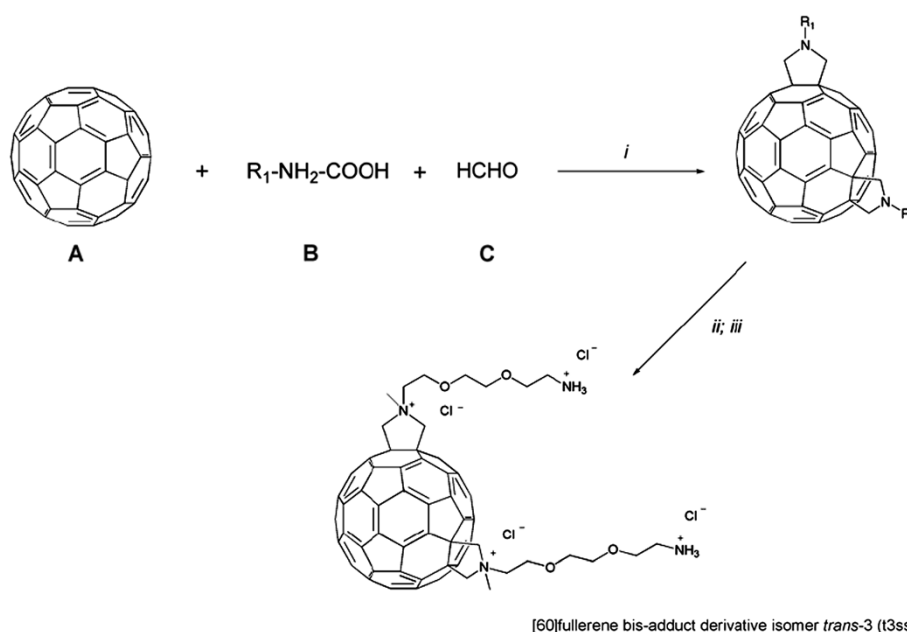
Figure 1 Synthetic scheme for trans -3 isomer [60]fullerene bis-adduct derivative (t3ss). R 1 = CH 2 CH 2 OCH 2 CH 2 OCH 2 CH 2 NHBoc. Reagent and conditions: (i) molar ratio A:B:C 1:2:5, toluene, 2 h at reflux, isolation of trans -3 isomer among the reaction mixture; (ii) CH 3 I, CH 2 Cl 2 , 24 h at 80°C; (iii) HCl (g), CH 3 OH, 20 min at 0°C. For more details and procedures see [20].
