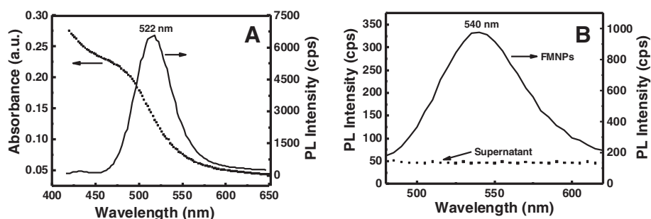
Figure 1 Spectroscopic analysis of CdTe QDs and FMNPs. (A) Absorbance and PL spectra of CdTe QDs; (B) PL spectra of FMNPs and supernatant solution.
