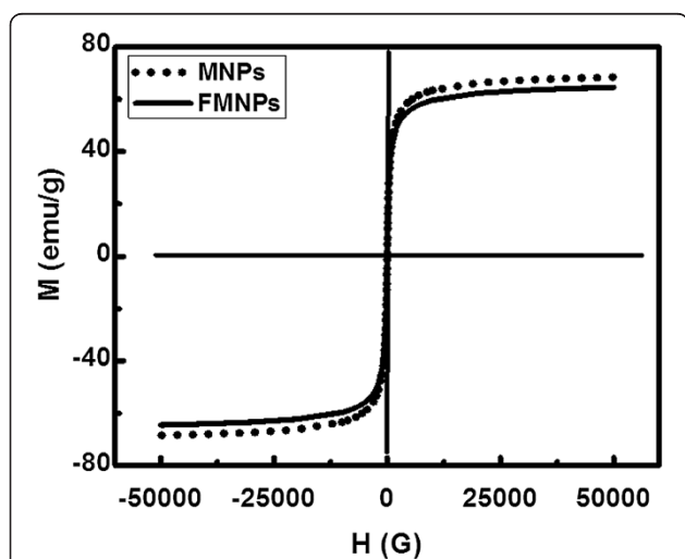
Figure 3 Hysteresis loops of the FMNPs. Magnetic properties of FMNPs and MNPs were measured using SQUID at 300 K.
