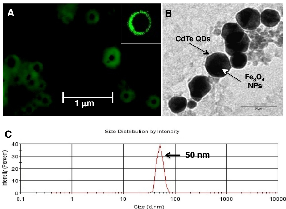
Figure 2 Images of TIRF (A) and TEM (B), and DLS (C). Bars in A and B denote 1 \mu\text{m} and 50 nm, respectively.
