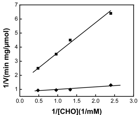
Figure 4 Lineweaver Burk plots of the initial rates of CHO (■) and (◆) \text{Fe}_3\text{O}_4 -CHO at pH 7.4, from experimental data.
